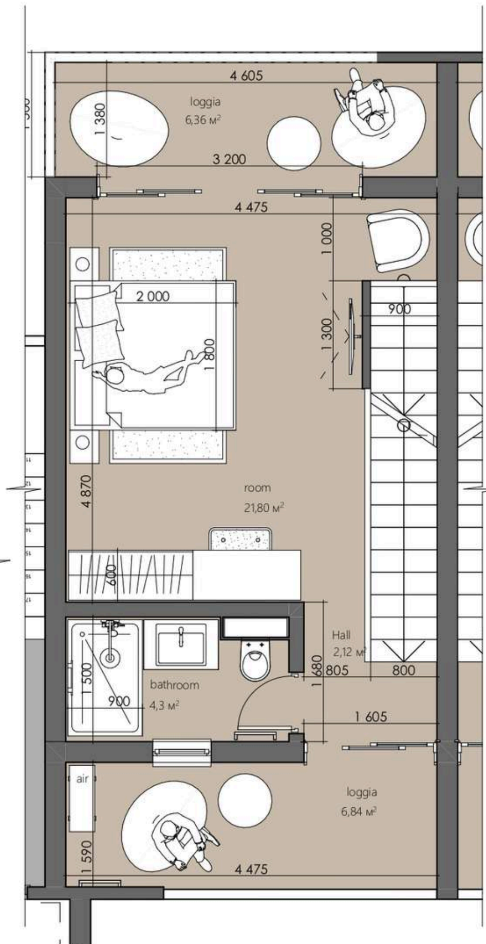
2nd floor
