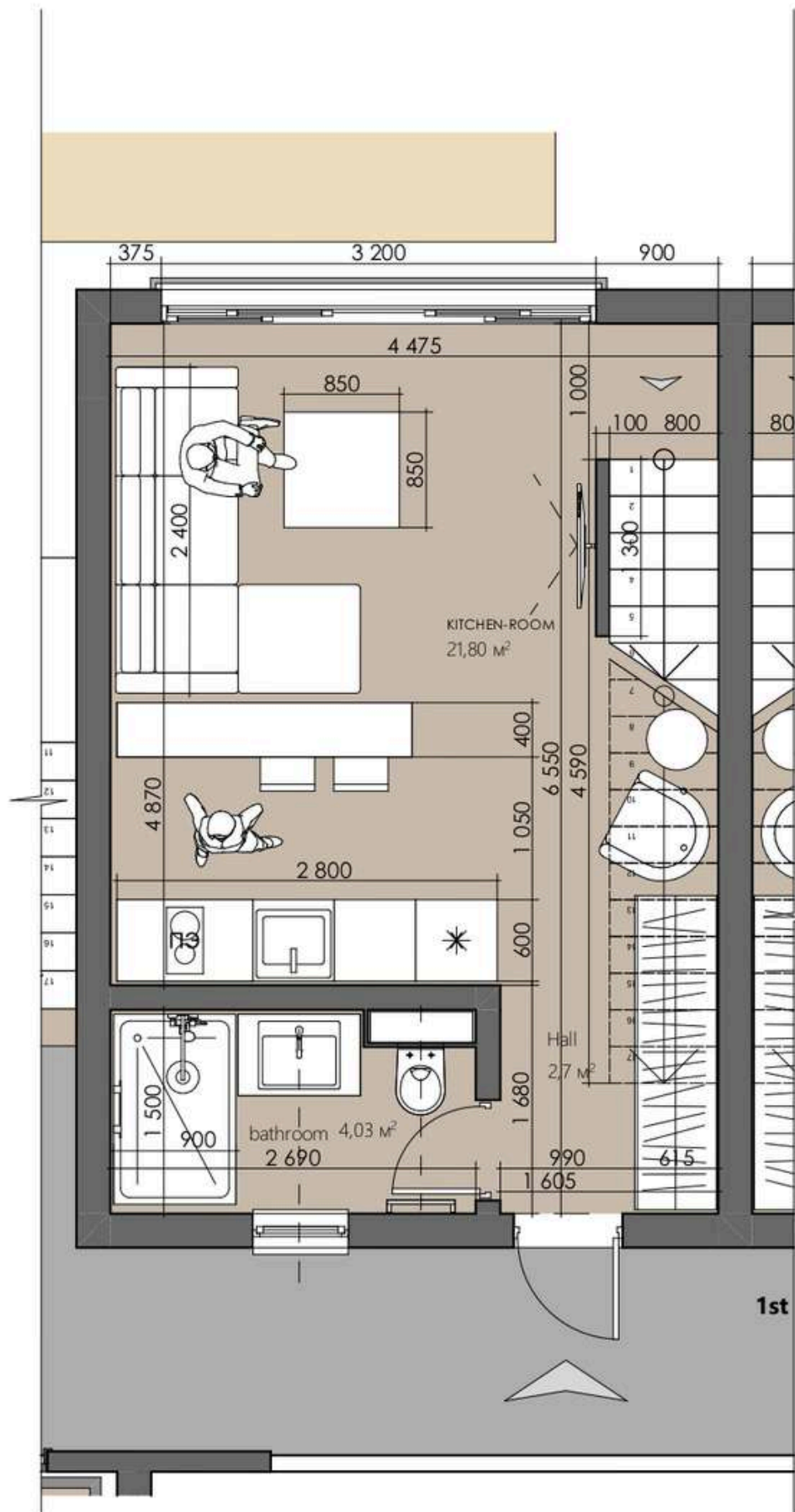
1st floor
