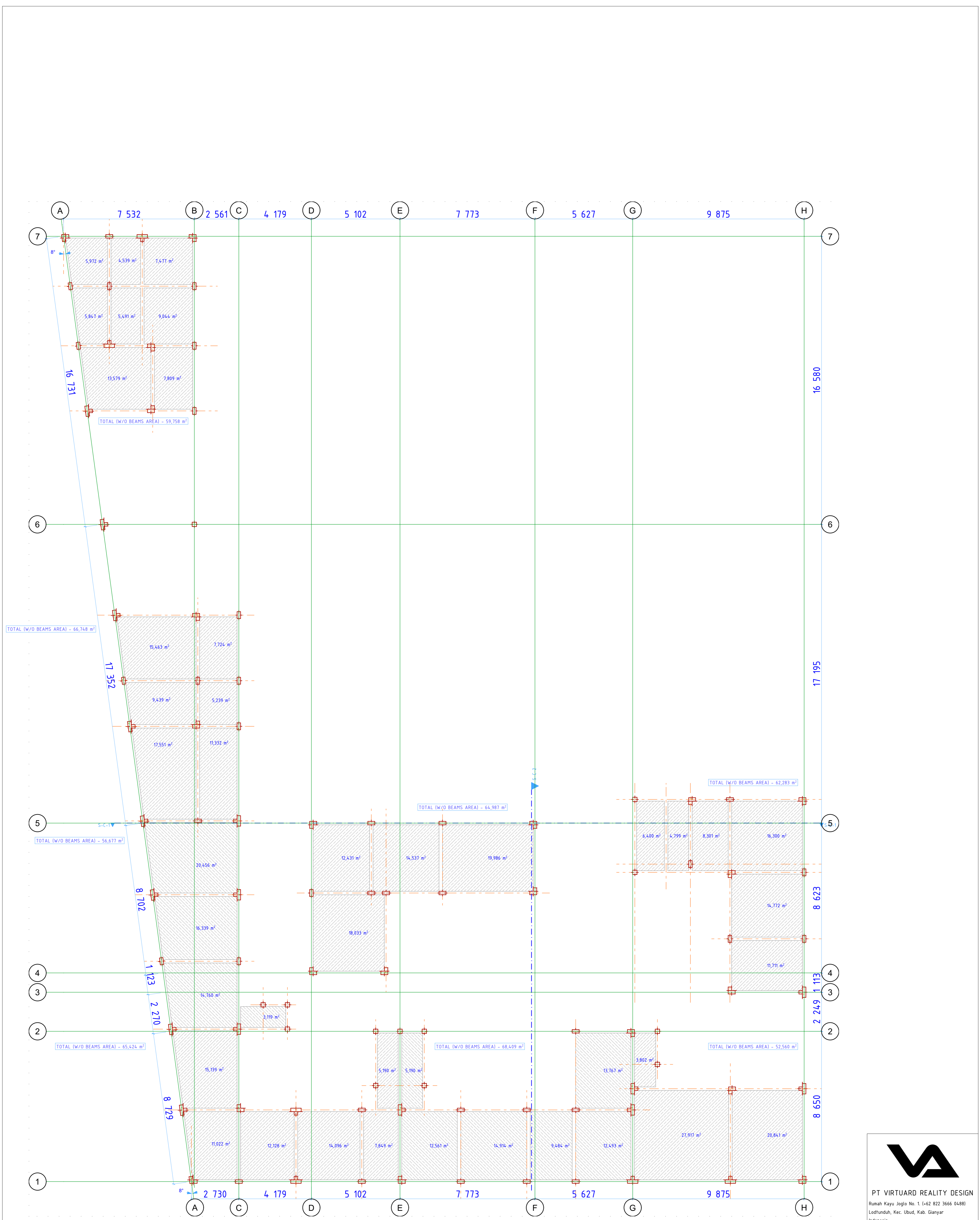
1. SLABS AREA 0 FLOOR 1:100
