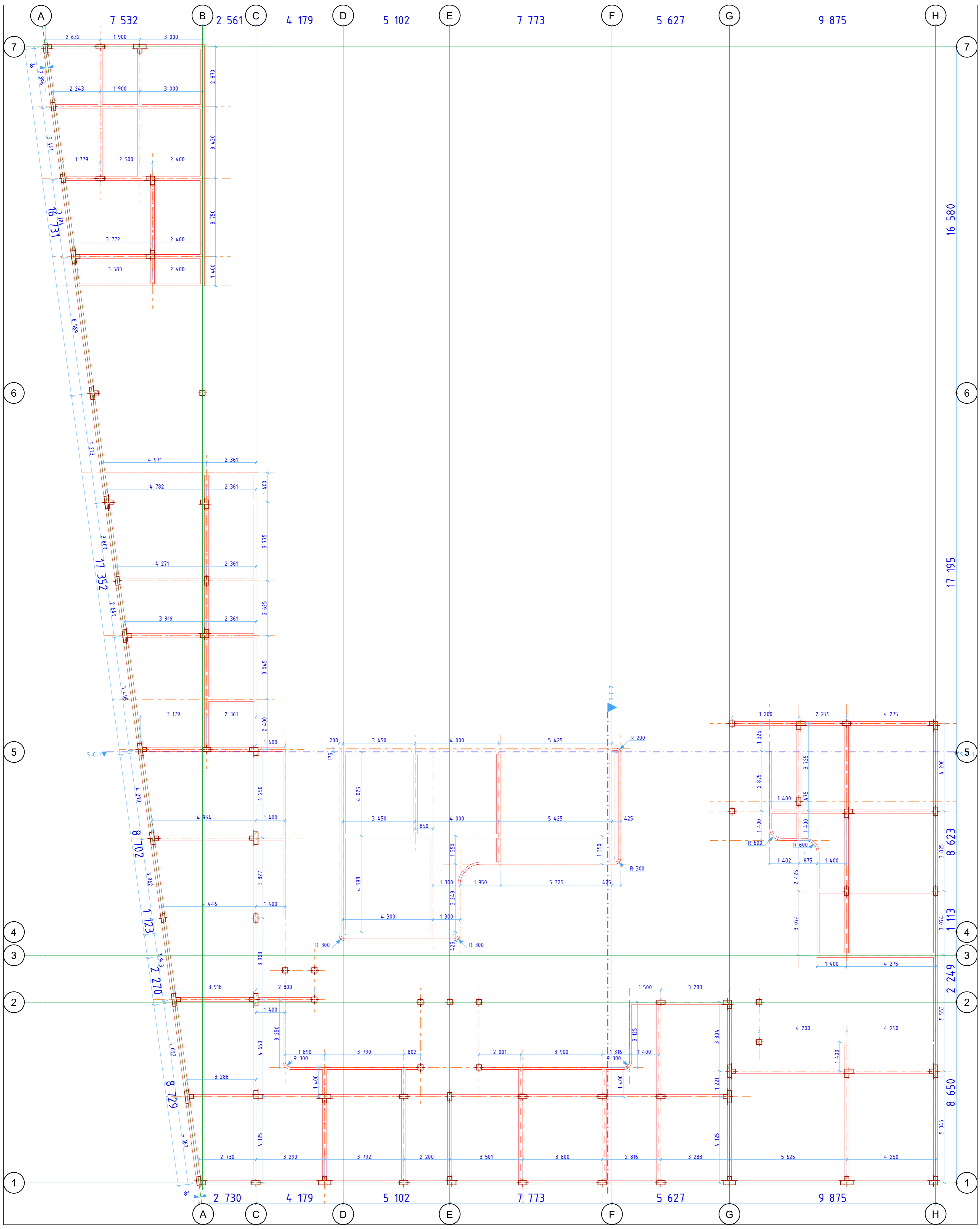
1. BEAMS DIMENSIONS 1 FLOOR 1:100
