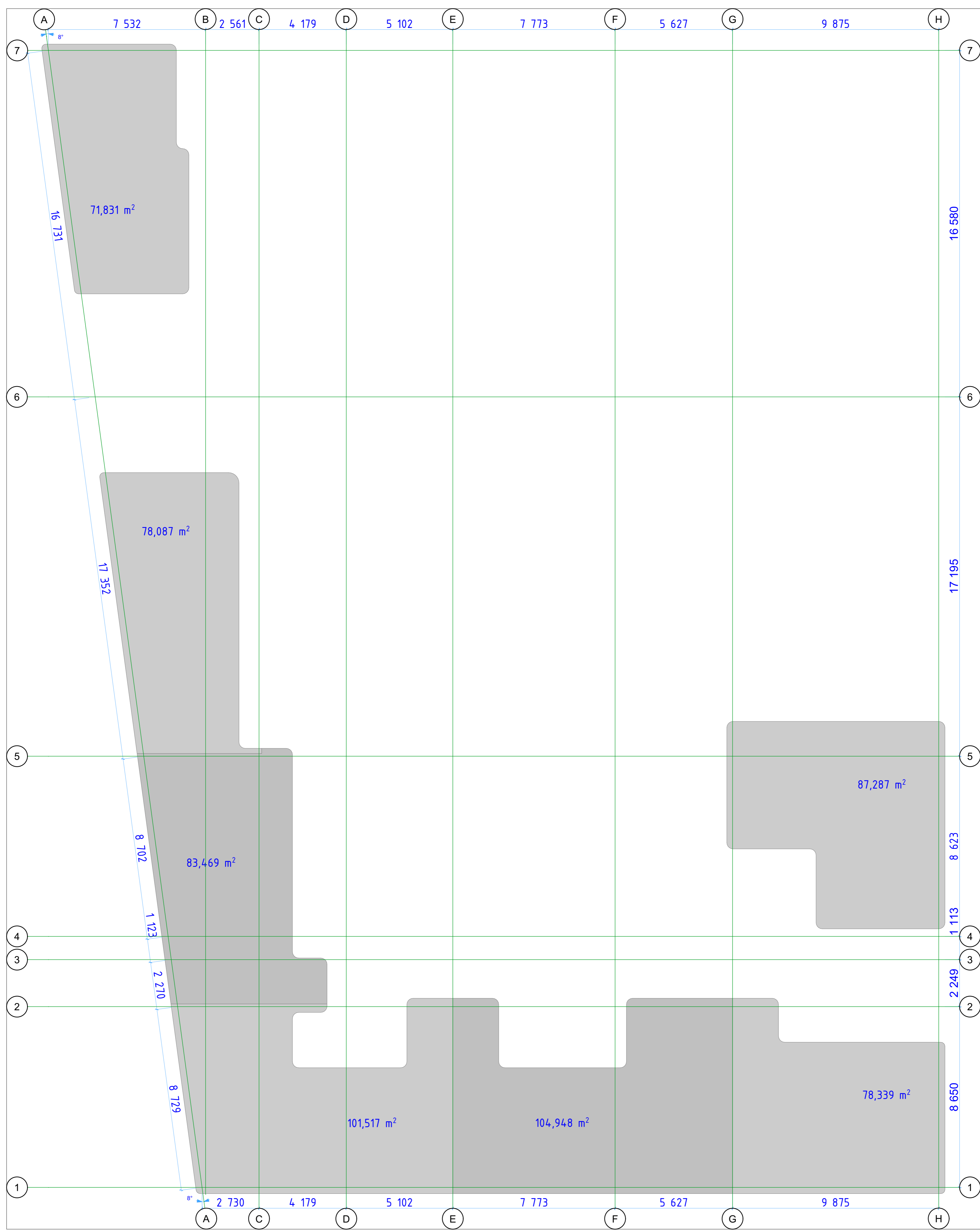
1. 2 FLOOR AREA 1:100
