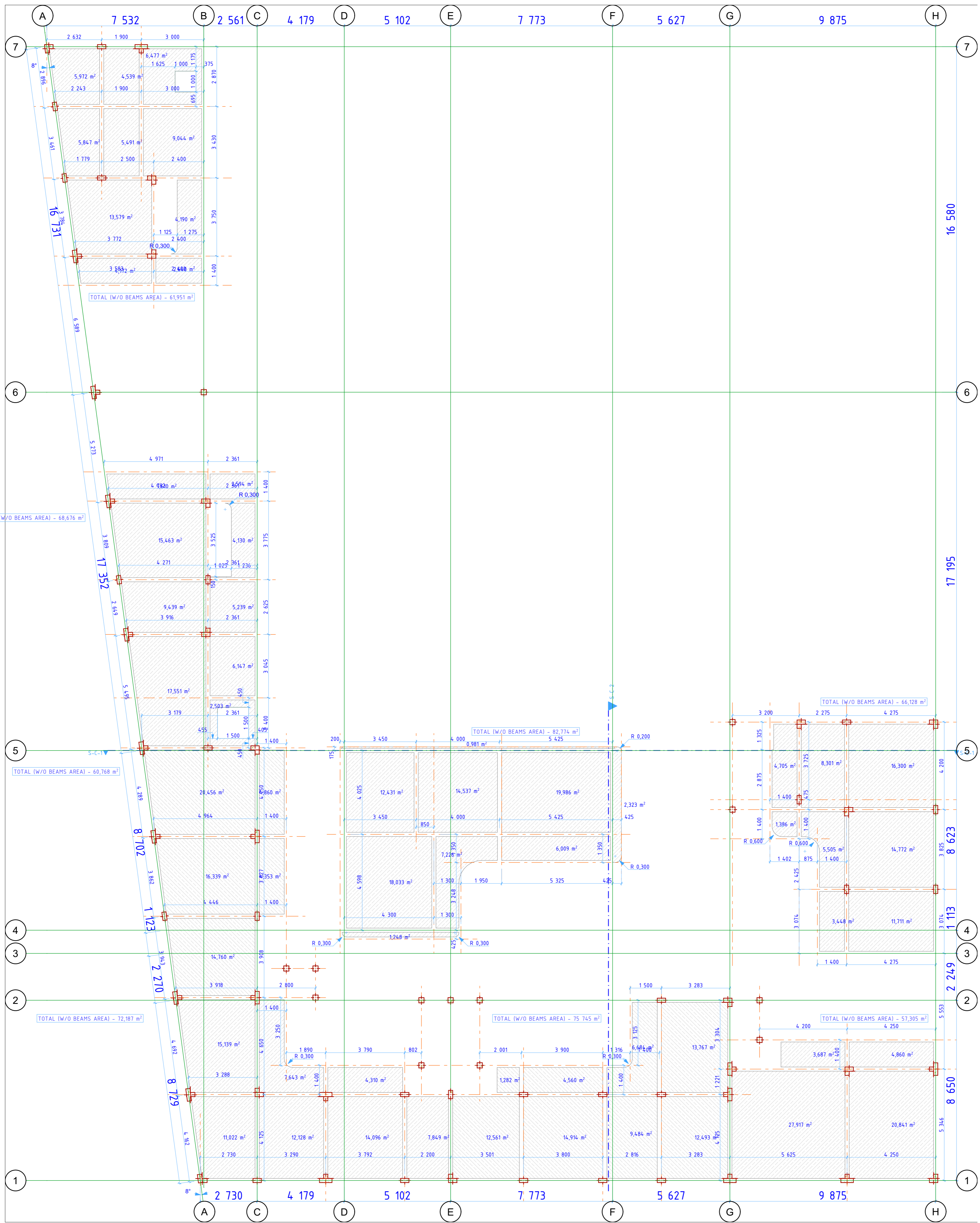
1. SLABS AREA 1 FLOOR 1:100
