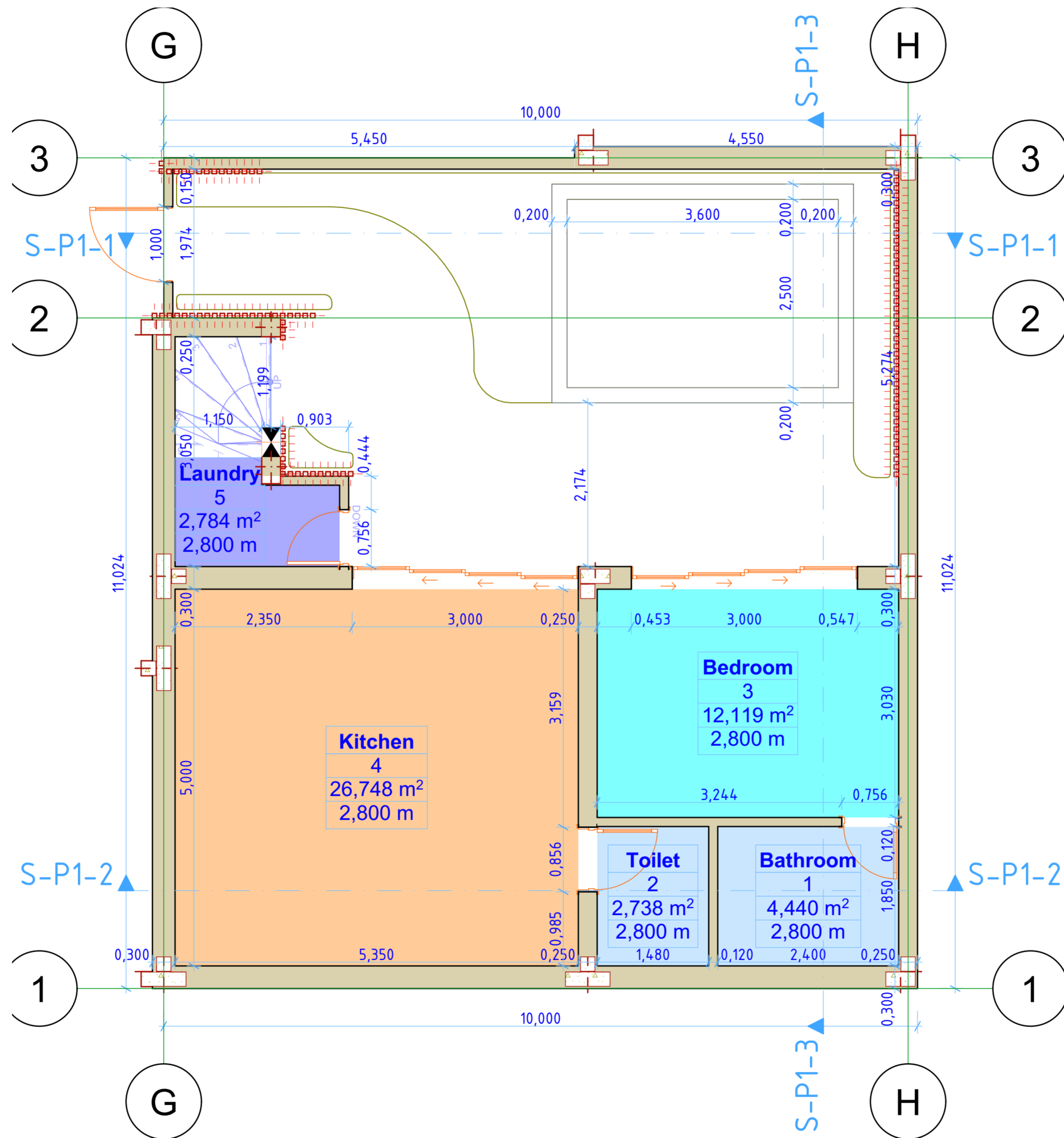
0. Plot 1 Floor 1 1:50
