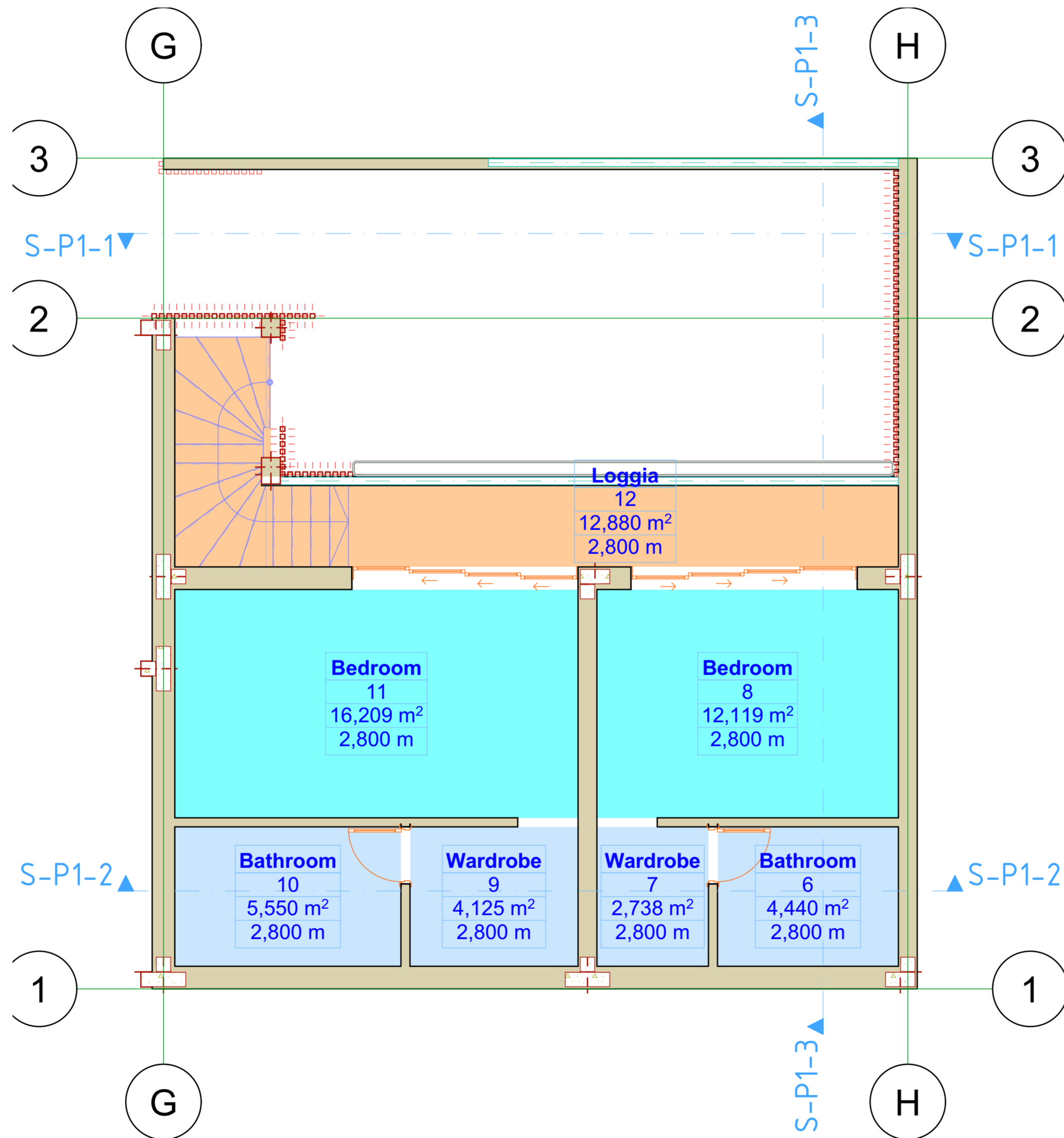
1. Plot 1 Floor 2 1:50
