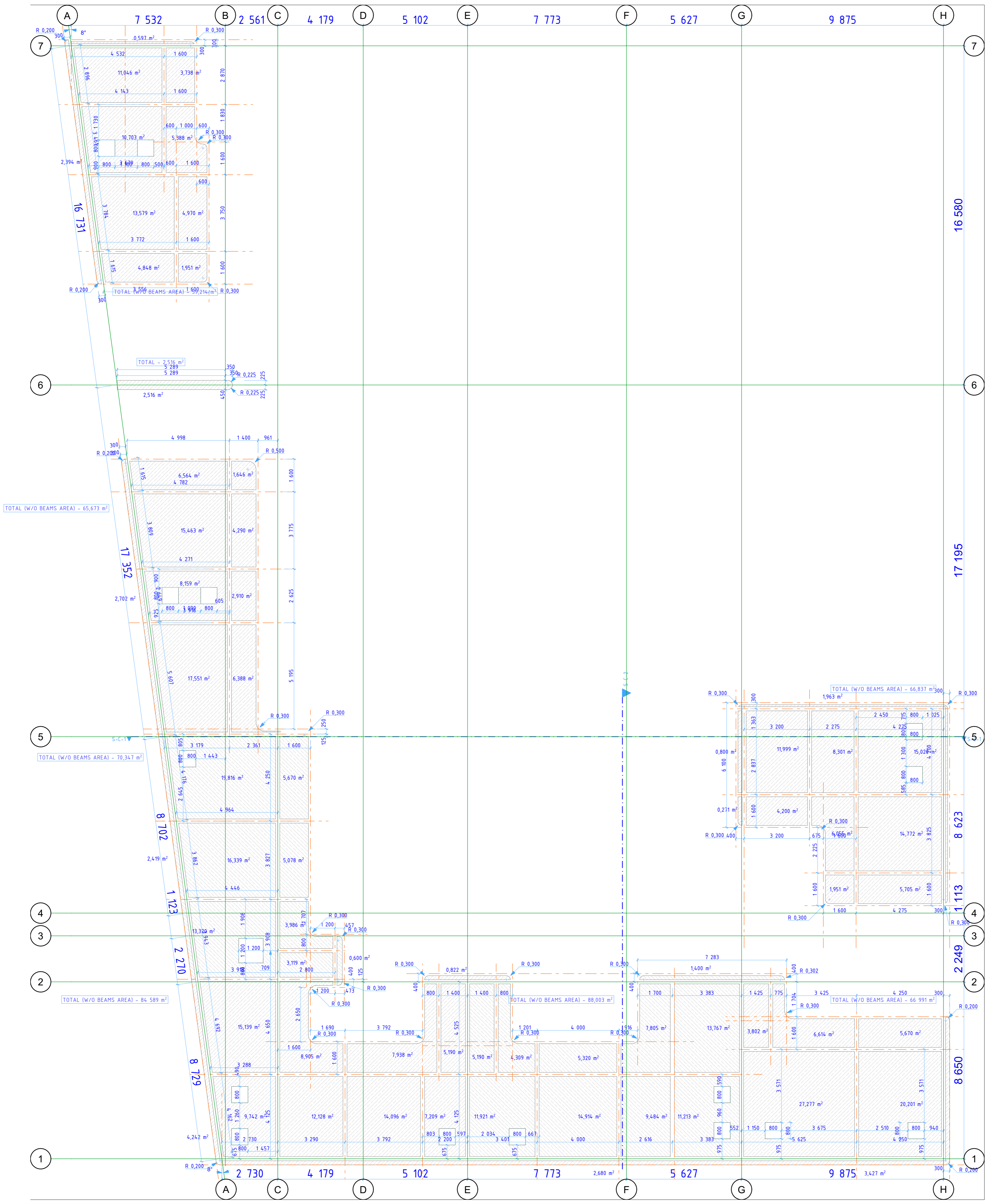
1. SLABS AREA 2 FLOOR 1:100
