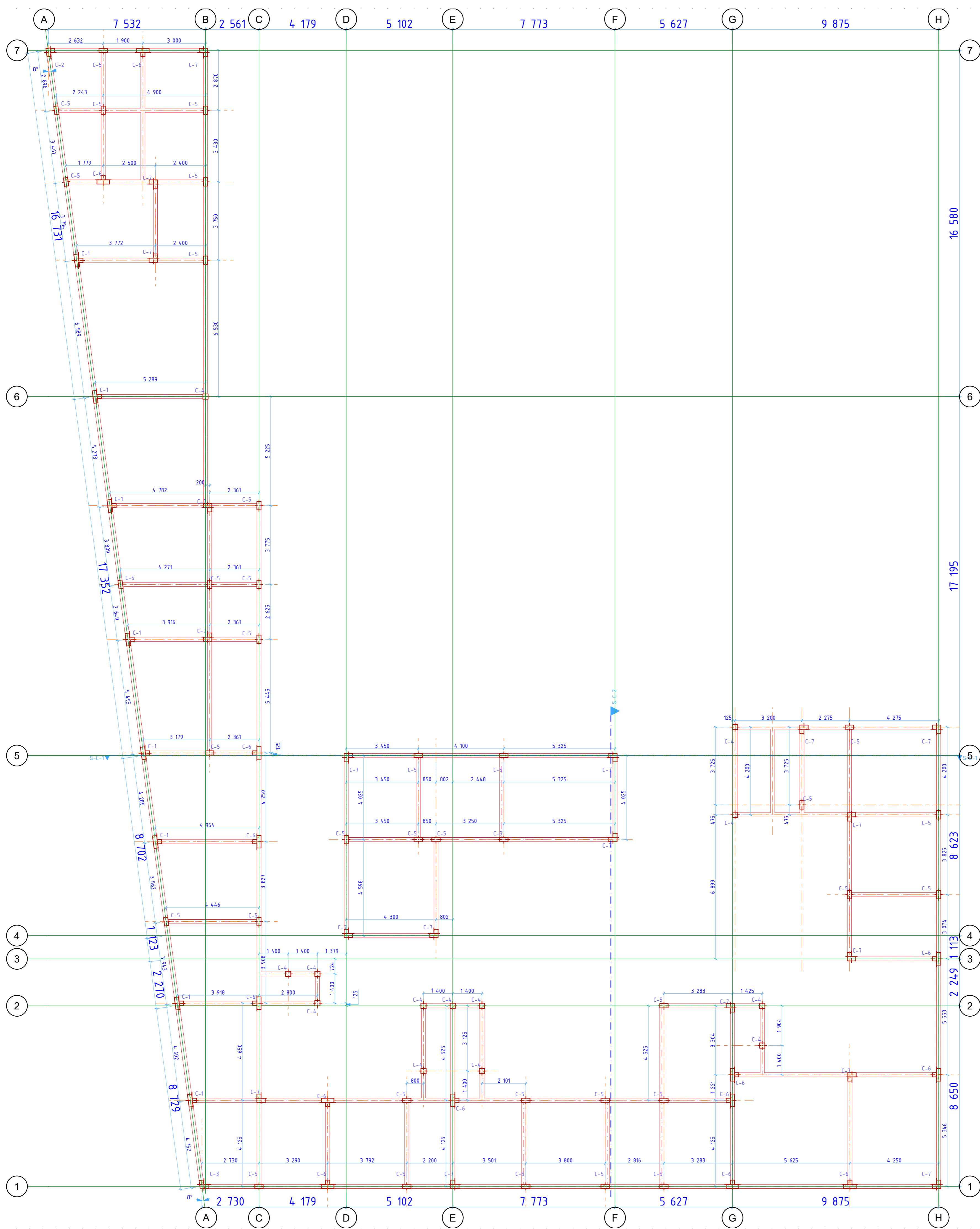
1. BEAMS DIMENSIONS 0 FLOOR 1:100
