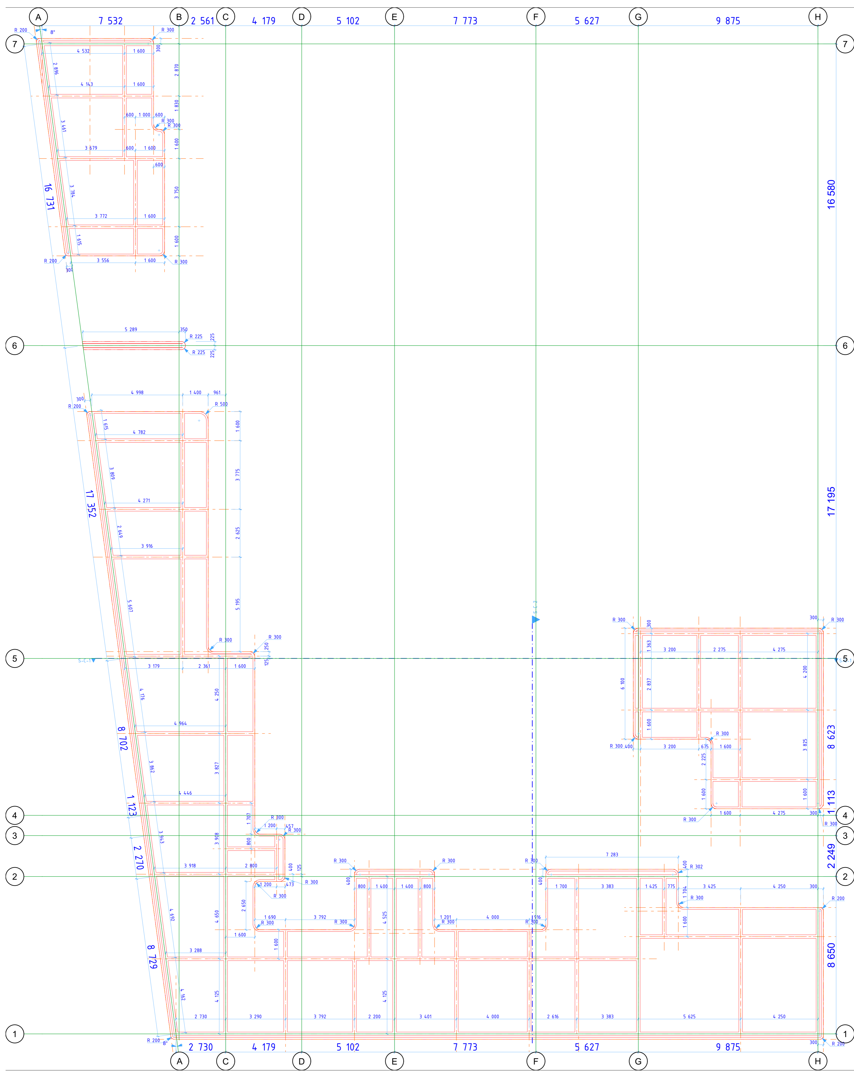
1. BEAMS DIMENSIONS 2 FLOOR 1:100
